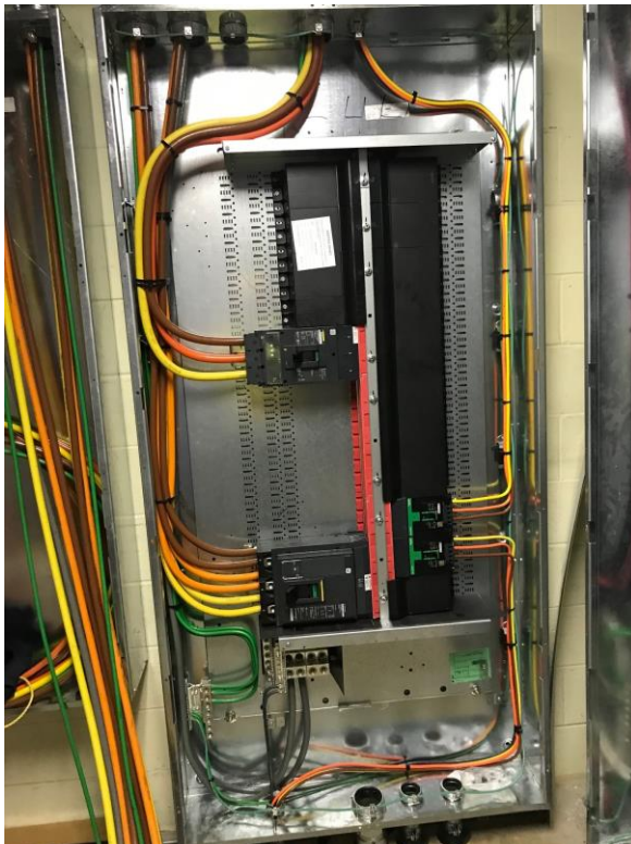
Panel Wiring
