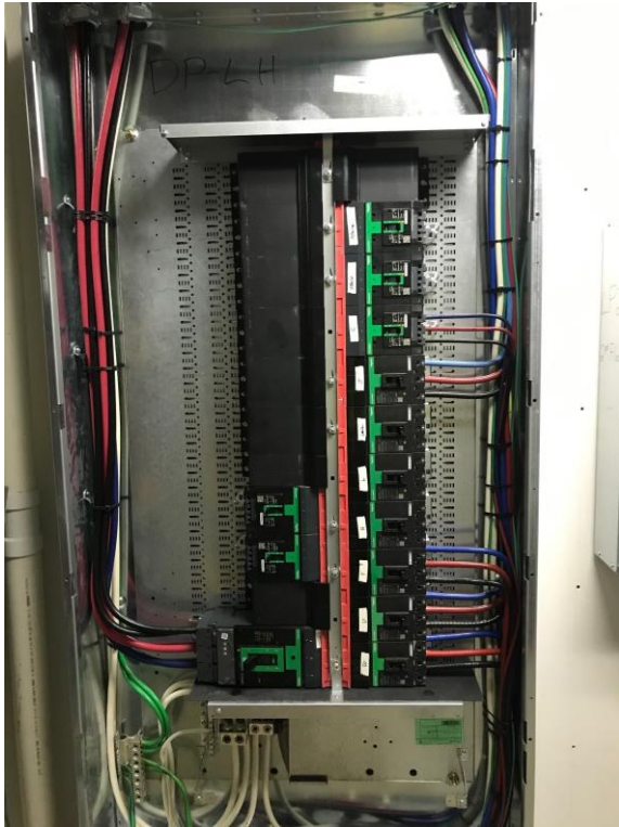
Panel Wiring
